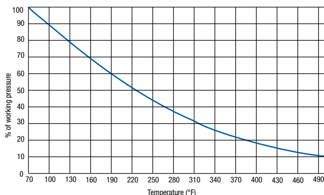
PFA Tubing (Series 104, 204) Maximum Working Pressure (bar)
